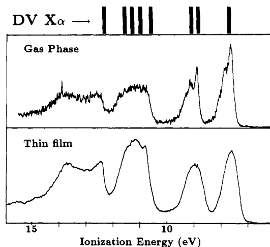
Figure 35. Gas phase (upper) and thin film (lower) He I valence photoelectron spectra of fullerene-60 obtained by Lichtenberger et al. 239,240 The DV- X_\alpha results of Hale 169 (see Figure 23) which appear to be in good agreement with observation are indicated (reprinted from ref 239; copyright 1991 Elsevier Science Publishers).
