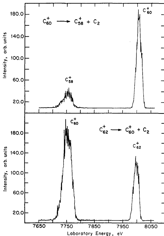
Figure 13. Metastable mass-analyzed ion kinetic energy scans (MIKES) published by Radi et al. 98 The parent ion (on the right) is mass selected by the magnetic analyzer and the horizontal axis is a scan of the electrostatic analyzer voltage. The parent ion energy is 8 keV. C 2 loss is observed from C 60 + (above) and C 62 + (below). Note the dramatic differences in metastable activity as reflected by the relative intensities of the product peaks, relative to their parent ions in these two cases (reprinted from ref 93; copyright 1990 the American Institute of Physics).
