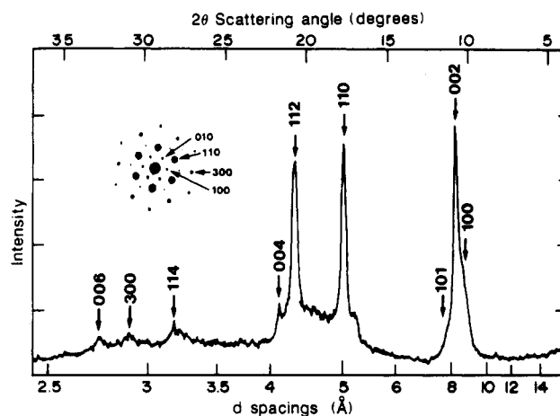
Figure 24. X-ray diffraction pattern of a microcrystalline powder of fullerene-60 obtained by Krätschmer, Lamb, Postropoulos, and Huffman. 4 Inset (upper left) is a single-crystal electron diffraction pattern (shown in more detail in Figure 25) indexed with Miller indices compatible with the X-ray pattern. This pattern provided unequivocal evidence that the C_{60} species they had isolated was a round ball 10 Å in diameter in perfect agreement with expectation for buckminsterfullerene (reprinted from ref 4; copyright 1990 Macmillan Magazines Ltd.).
